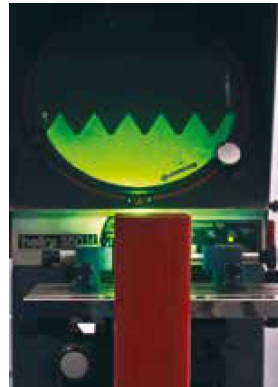
Thread Ring checking on SIP Universal Length measuring instrument.
